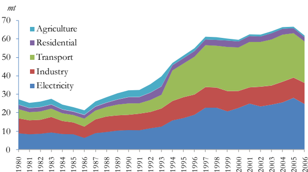
Figure 6: CO 2 Emissions From Fossil Fuels
