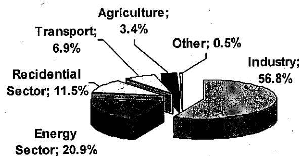
Figure 4.1 Structure of Energy-Efficiency Potential
