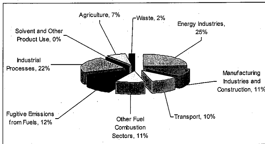
Figure 2.1 Emissions by Sector in Ukraine, 2006
