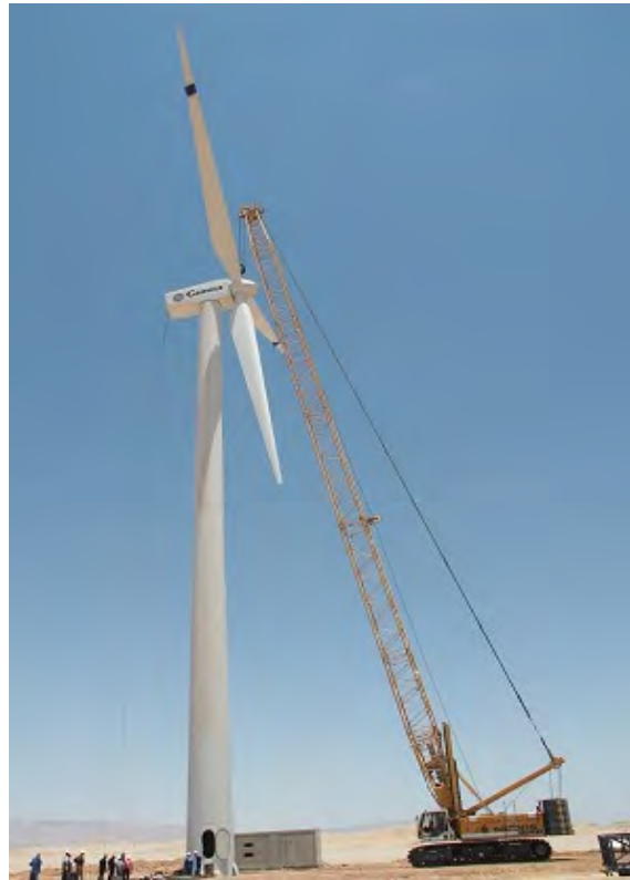
Photo: Erection of a Wind Turbine at Zafarana
