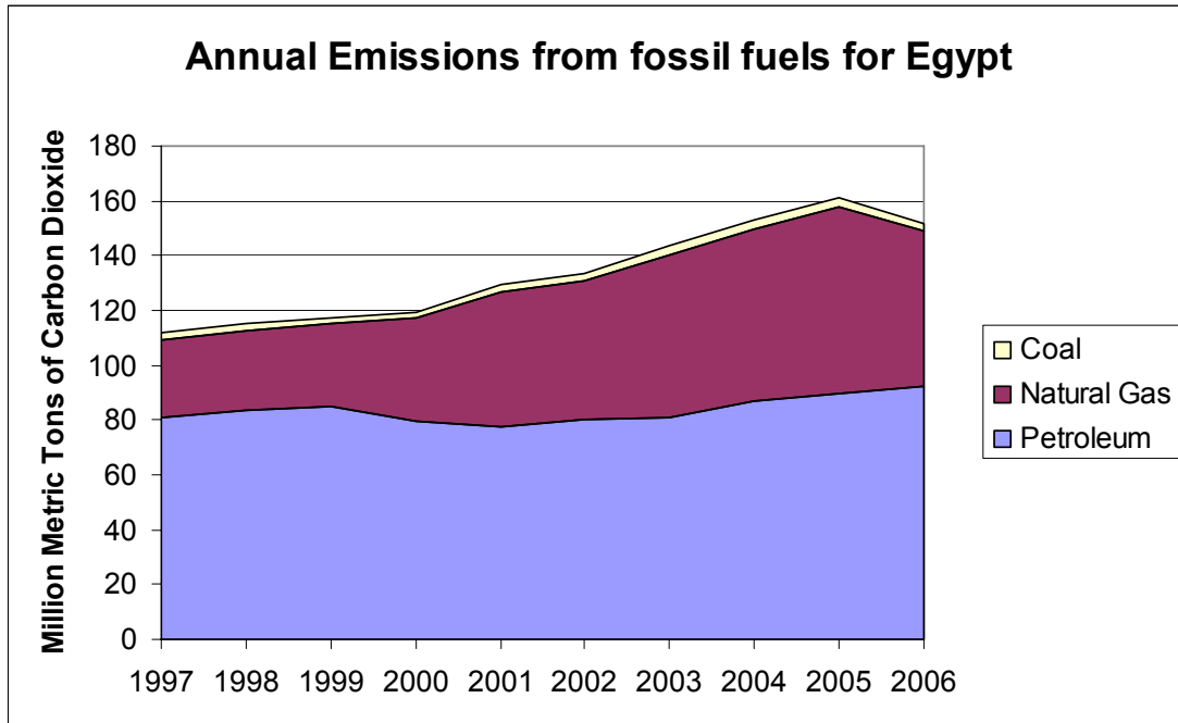
Figure 1: Annual Emission from Fossil Fuels
