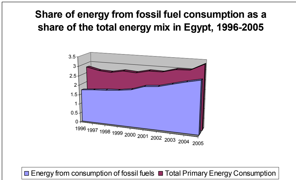
Figure 2: Share of Fossil Fuels in Total Primary Energy Consumption
