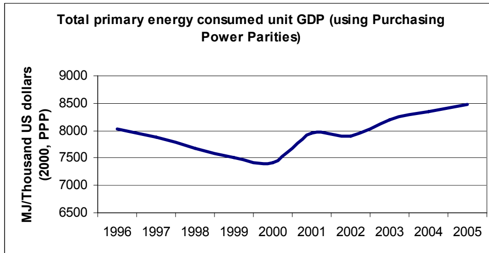
Figure 3: Total Energy Consumed per Unit of GDP
