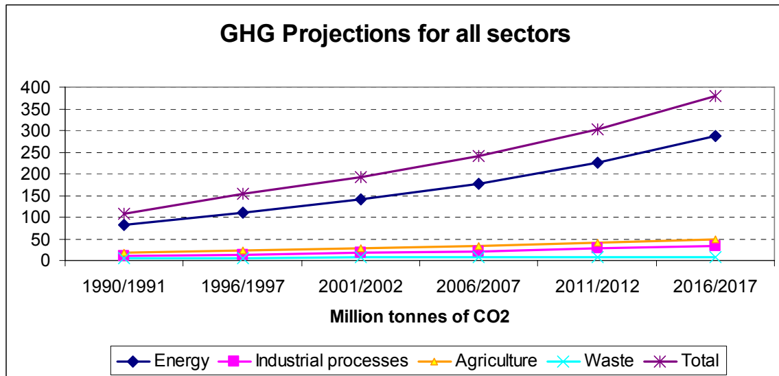
Figure 5: GHG Emissions by Sector
