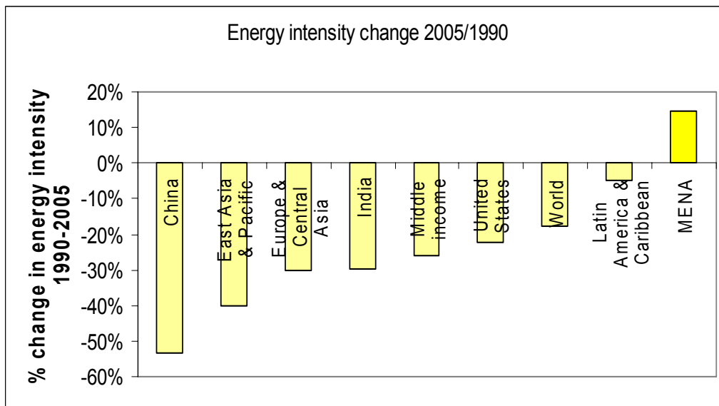
Figure 4: Energy Intensity change 2005/1990
