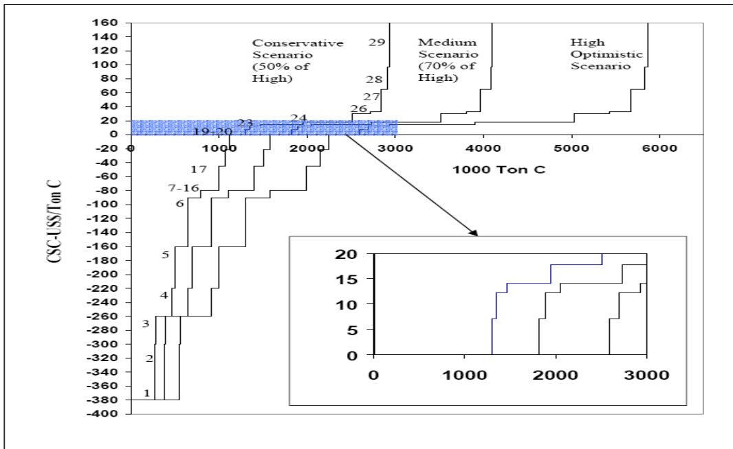
Figure 6: Marginal Abatement Cost Curve
